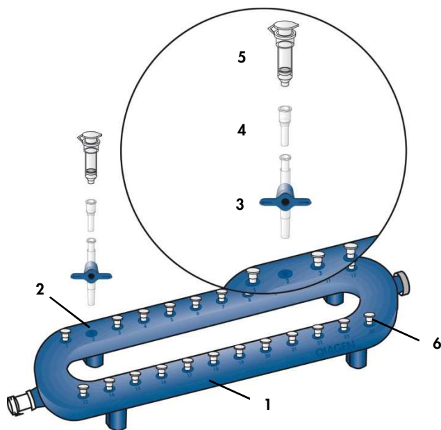
Figure 2. Setting up the QIAvac 24 Plus with QIAamp Mini columns using VacValves and VacConnectors. 1 = QIAvac 24 Plus vacuum manifold; 2 = Luer slot of the QIAvac 24 Plus; 3 = VacValve (optional; must be purchased separately); 4 = VacConnector (must be purchased separately); 5 = QIAamp column; 6 = Luer slot closed with luer plug.
